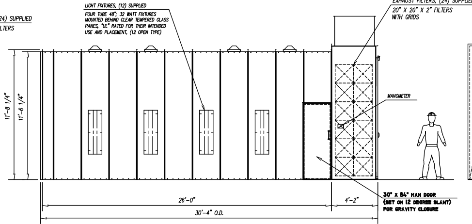
BOOTH SIDE VIEW
