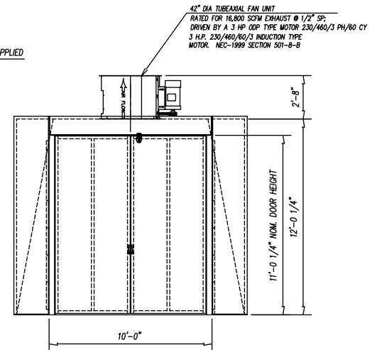
END VIEW @ CHAMBER
