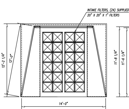
END VIEW FROM BAY END
